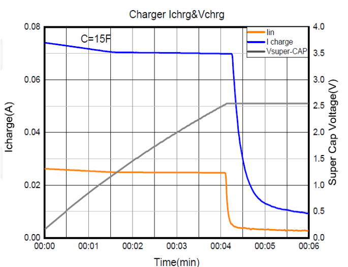
Figure 7 Charger Icharg&chrg
