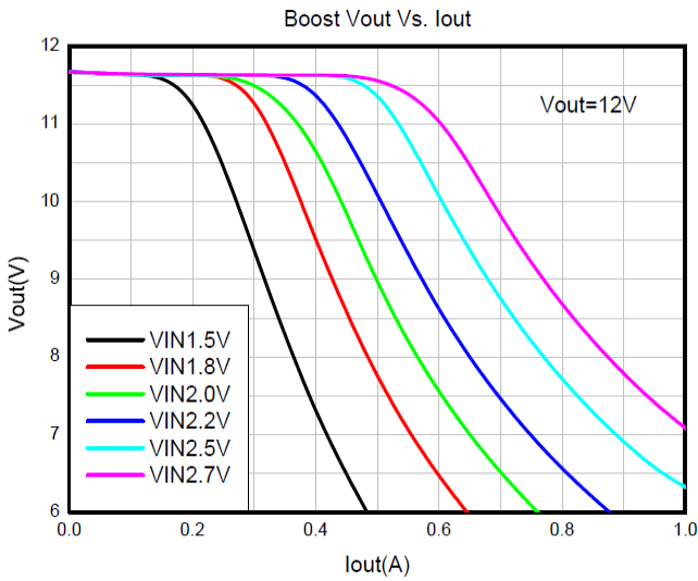
Figure 2 Boost Vout Vs. Iout
