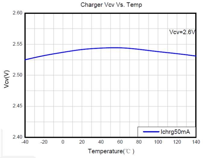
Figure 9 Charger Vcv Vs.Temp
