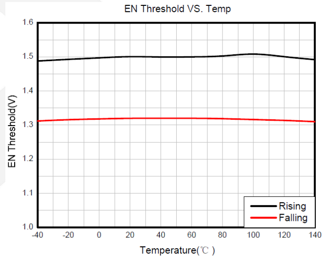
Figure 11 EN Threshold Vs.Temp
