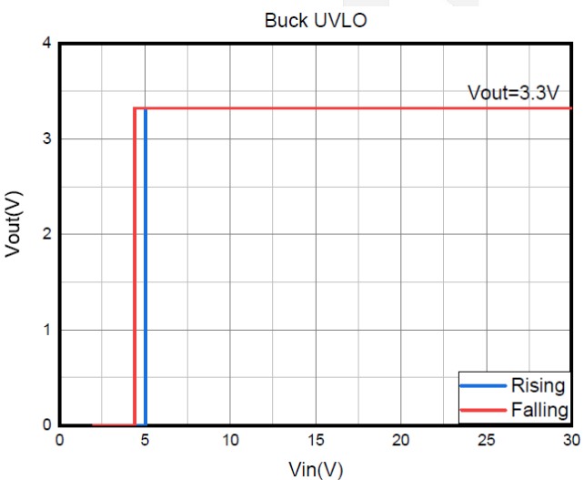
Figure 6 Buck UVLO
