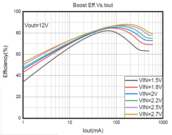
Figure 3 Boost Eff.Vs.Iout
