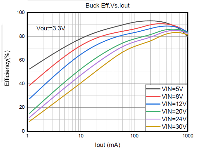
Figure 5 Buck Eff.Vs.Iout
