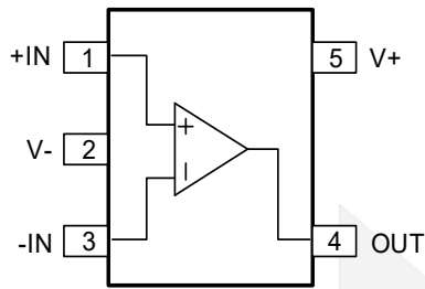
SC70-5
