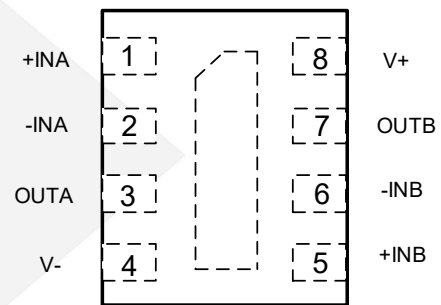
DFN1.6*1.2-8
