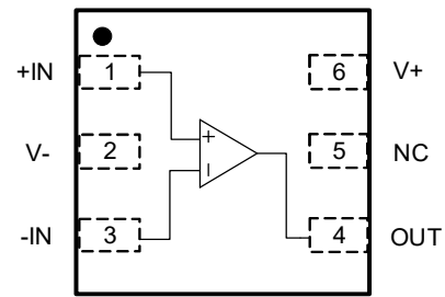
DFN1*1-6
