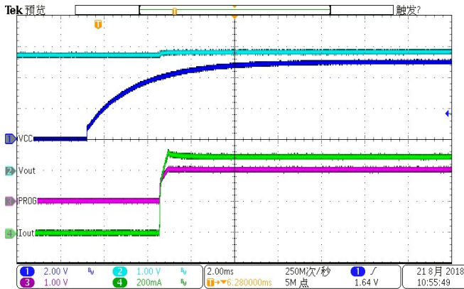
Charging Curve
